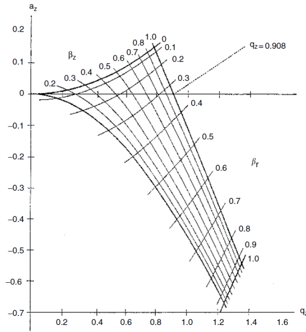
Figure 1-3. Stability diagram near origin in a conventional quadrupole ion trap. (Adapted from March, R.E.; Todd, J. F. J., Quadrupole Ion Trap Mass Spectrometry , John Wiley & Sons, Inc., 2005, pp 34-72.)
