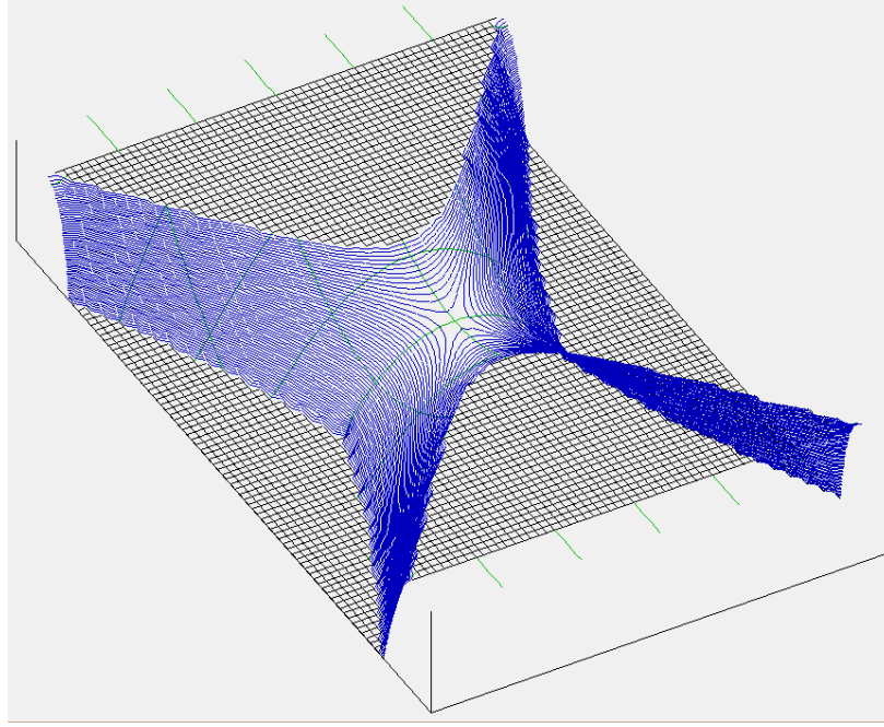
Figure 1-2. Quadrupolar field in a quadrupole ion trap. The four poles of the potential surface vary with time at a static trapping frequency.
